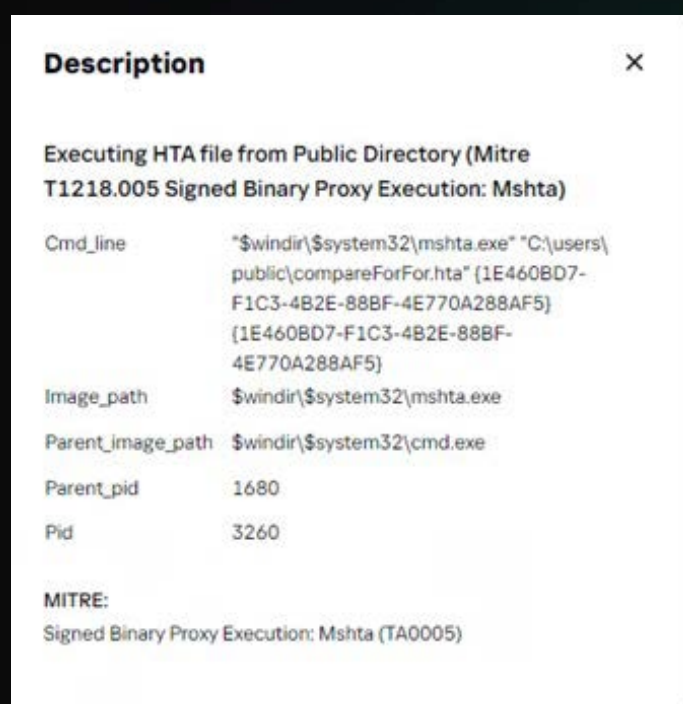
Fig. 19 — Suspicious activity: Conti. mshta.exe
